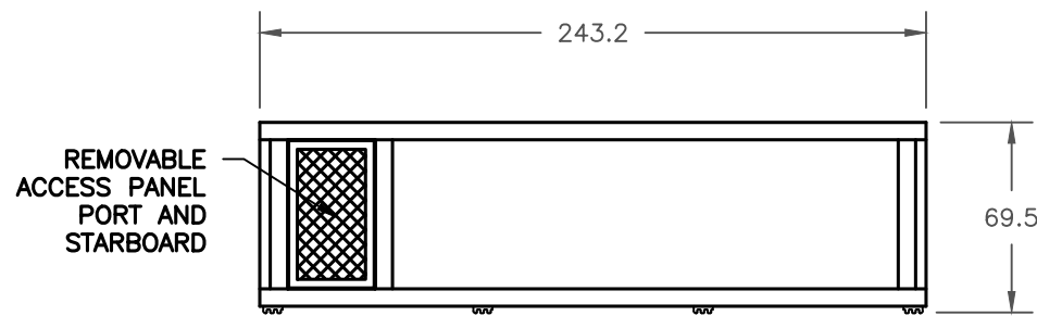
STARBOARD VIEW
