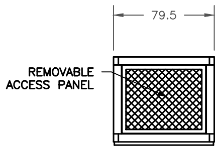
STERN VIEW
