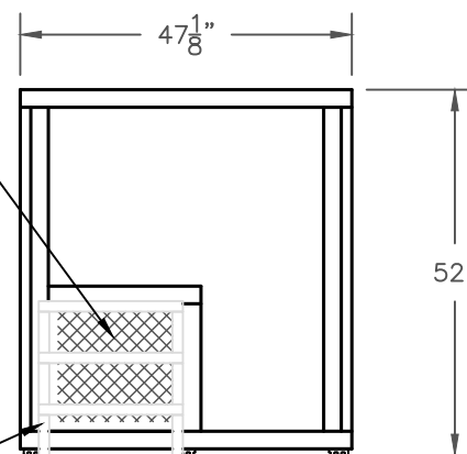
STARBOARD VIEW with STEPS
