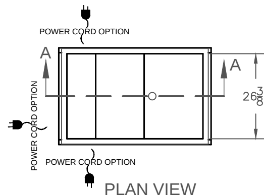
SETBACK VIEW
