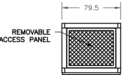
STERN VIEW
